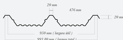
TRAPEZOIDAL TP 100/950
